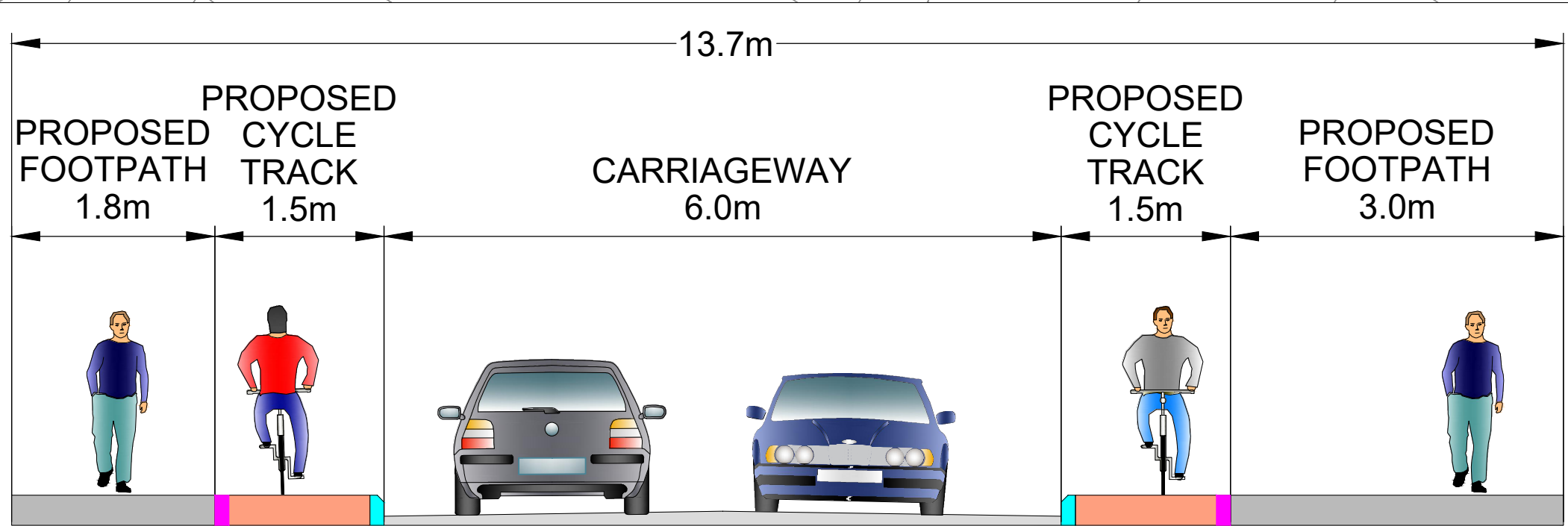
CROSS SECTION N-N
